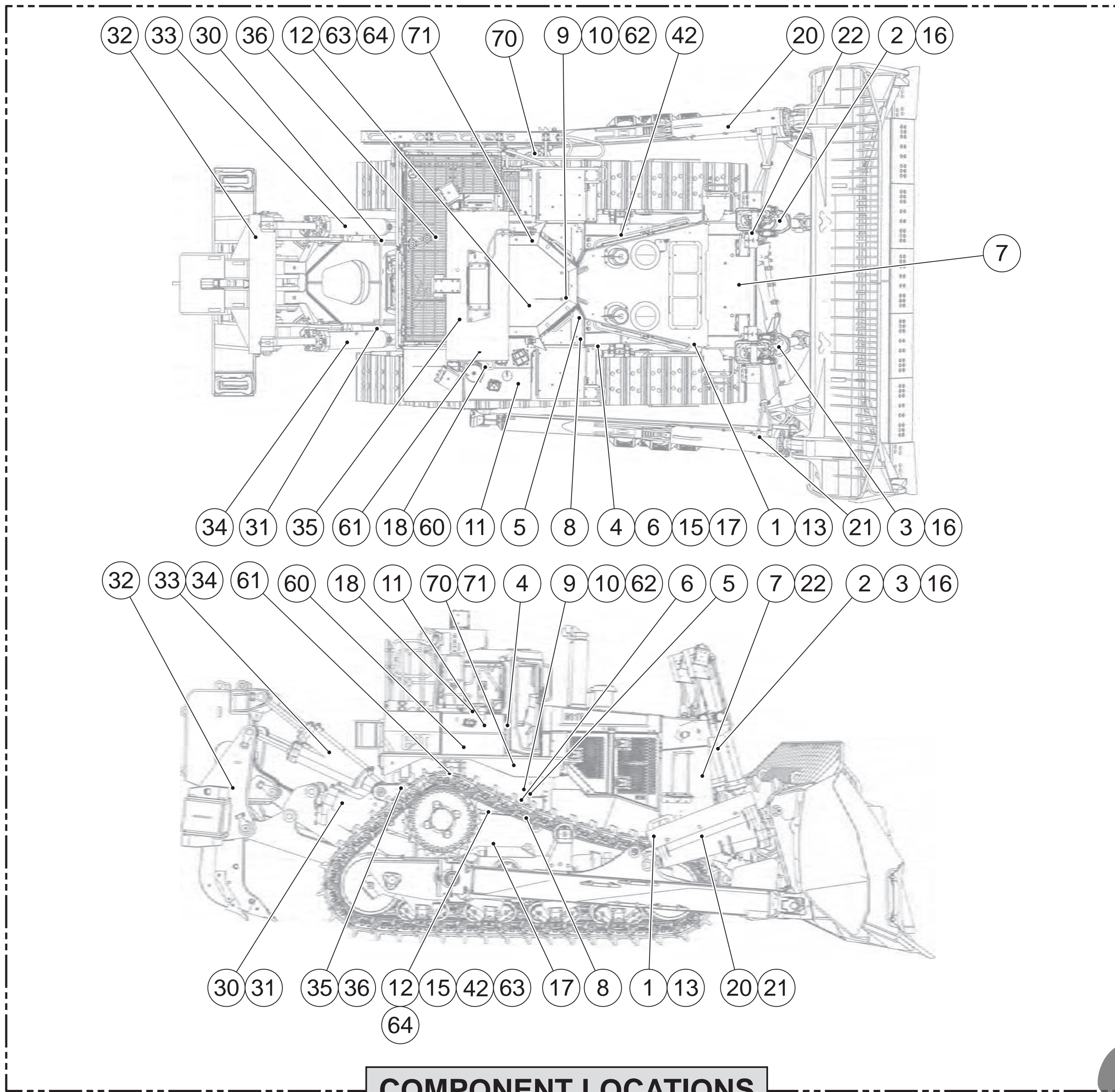
COMPONENT LOCATIONS
